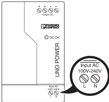
Bild 6 Screw connection for input AC L/N
